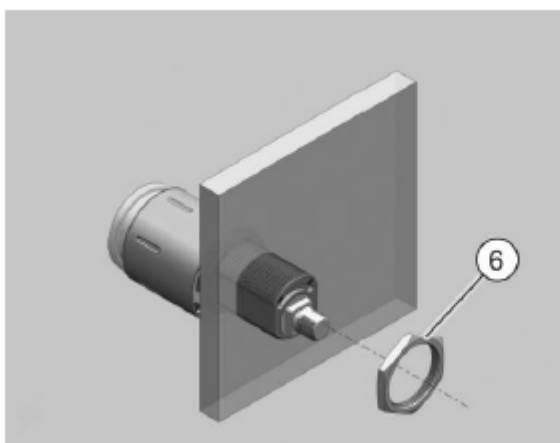
Fig. 147: Securing the cylinder with the hexagon nut
