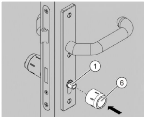
Fig. 14: Fitting the inner knob
