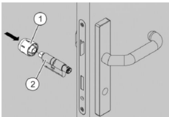
Fig. 91: Fitting the inner knob
