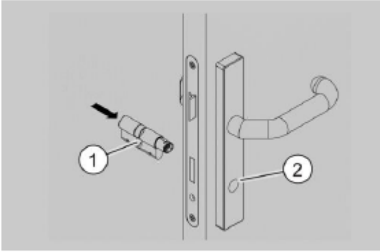
Fig. 121: Inserting the cylinder
