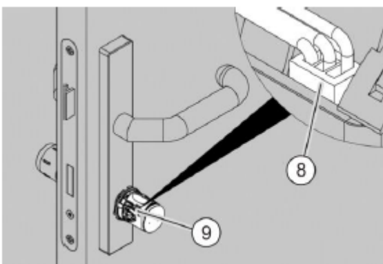
Fig. 48: Connecting the battery
