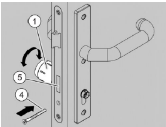
Fig. 69: Aligning the locking nose
