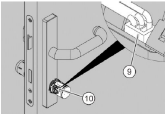
Fig. 22: Connecting the battery
