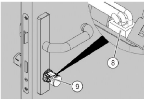
Fig. 40: Connecting the battery
