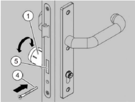
Fig. 85: Aligning the locking nose
