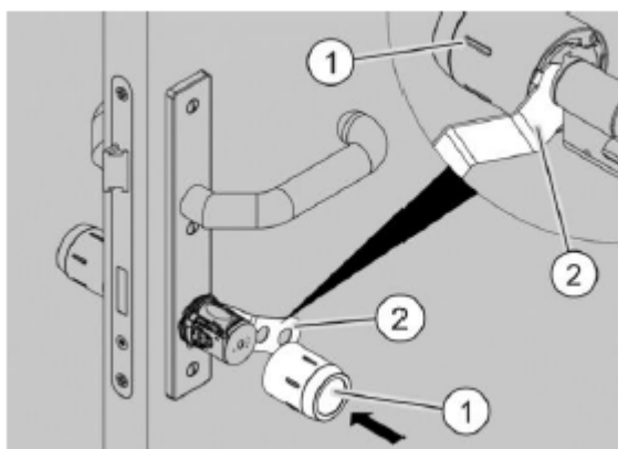
Fig. 164: Assembling the knob sleeve
