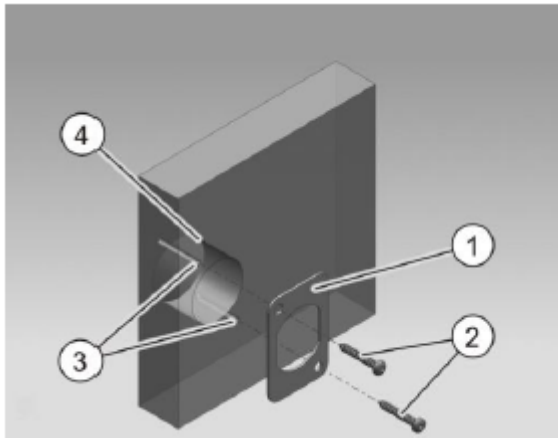
Fig. 145: Preparing the door with a retaining plate
