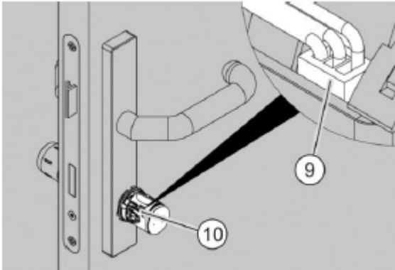
Fig. 78: Connecting the battery
