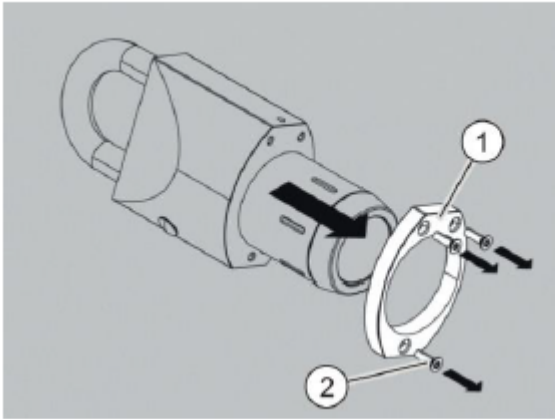
Fig. 168: Dismantling the protective cap
