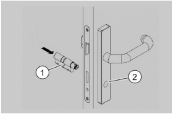
Fig. 107: Inserting the cylinder
