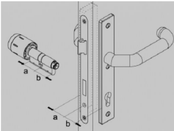
Fig. 28: Measuring the thickness
