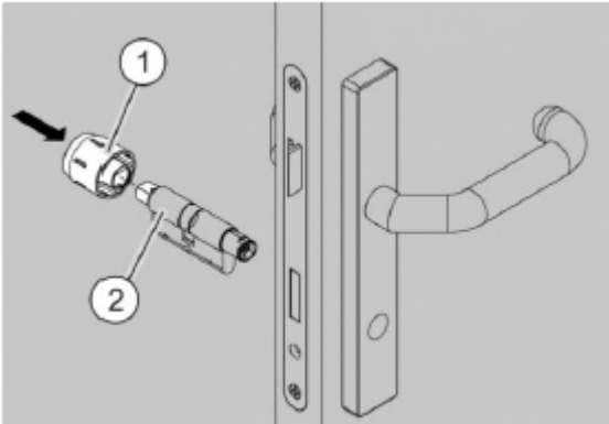
Fig. 73: Fitting the inner knob
