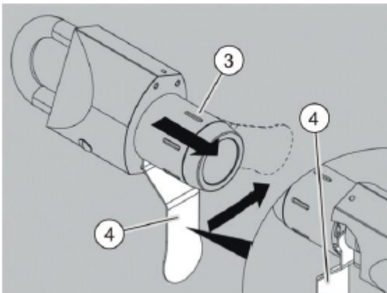
Fig. 169: Dismantling the knob sleeve
