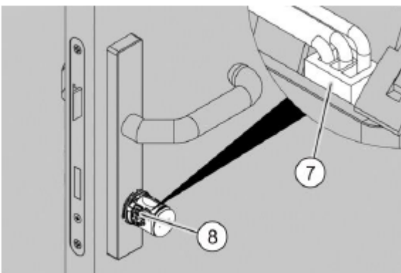
Fig. 124: Connecting the battery
