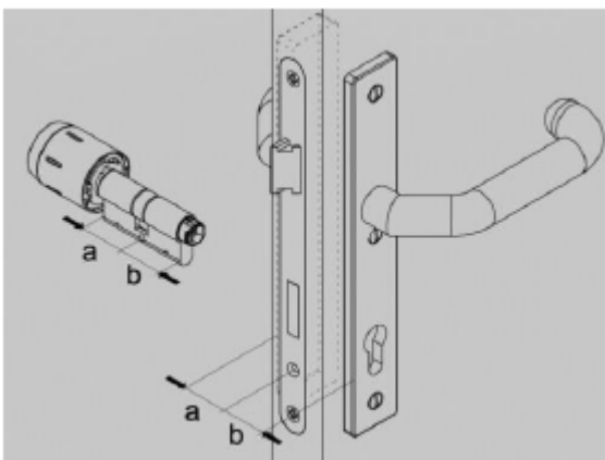
Fig. 44: Measuring the thickness
