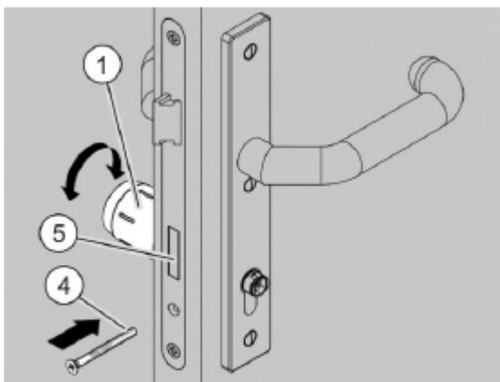
Fig. 38: Inserting the cylinder
