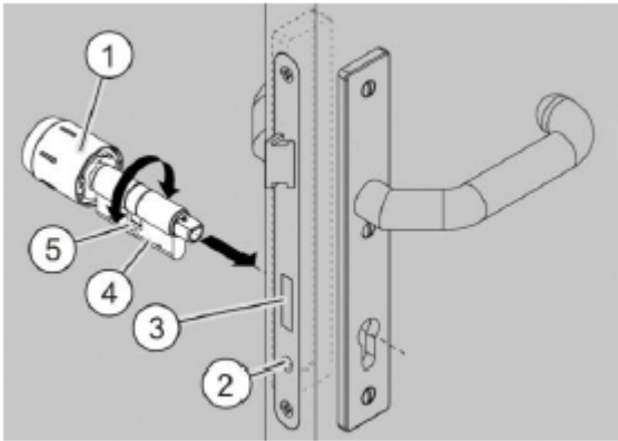
Fig. 117: Inserting the cylinder
