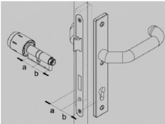
Fig. 72: Measuring the thickness
