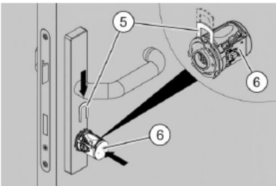
Fig. 123: Assembling the electronic knob
