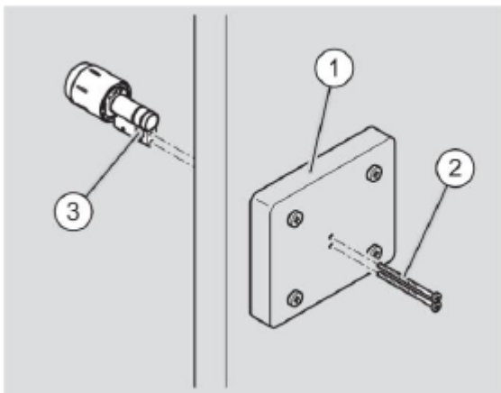
Fig. 141: Assembling the cylinder
