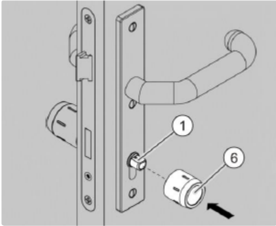
Fig. 55: Fitting the inner knob
