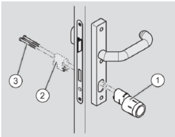
Fig. 155: Assembling the cylinder
