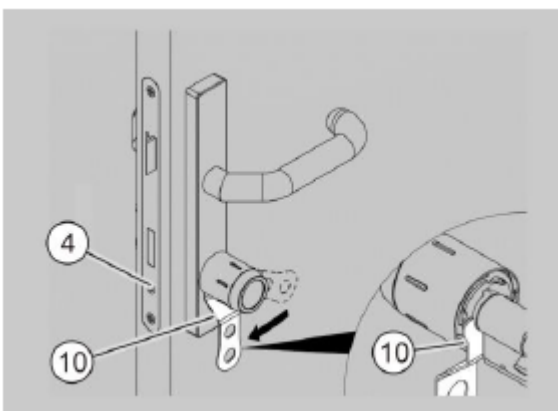
Fig. 113: Locking the bayonet lock
