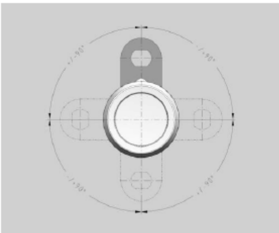
Fig. 150: Selecting the lever perforations
