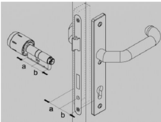
Fig. 36: Measuring the thickness
