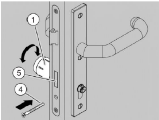
Fig. 54: Aligning the locking nose
