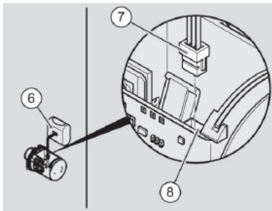
Fig. 135: Connecting the battery
