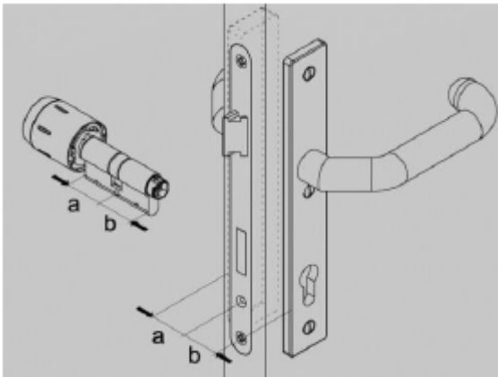
Fig. 11: Measuring the thickness
