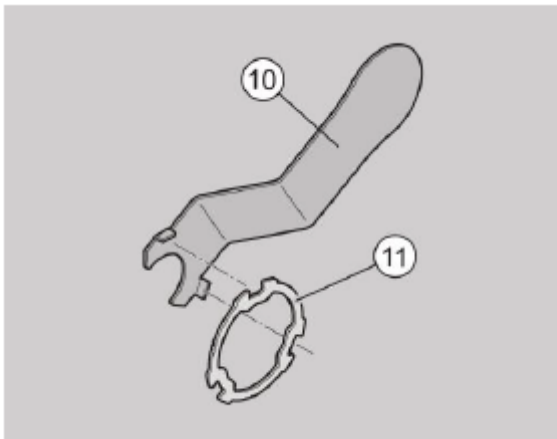
Fig. 126: Attaching the knob tool
