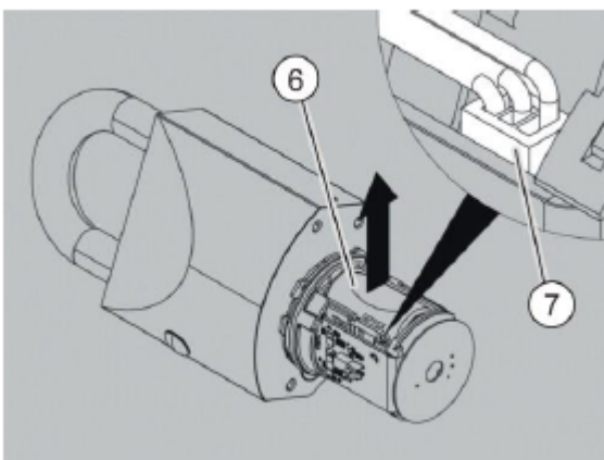
Fig. 171: Removing the battery pack
