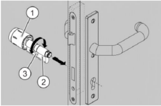
Fig. 37: Aligning the locking nose
