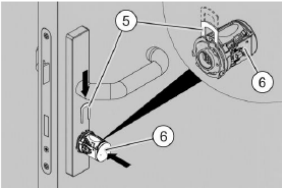
Fig. 31: Assembling the electronic knob
