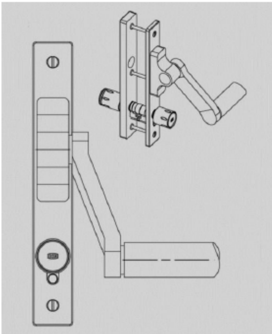
Fig. 115: Installation situation for the panic bar
