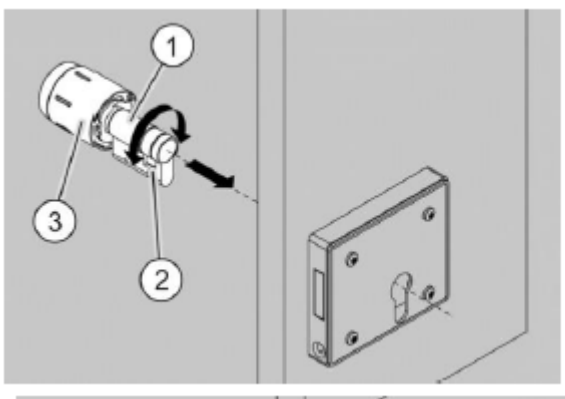
Fig. 130: Aligning the locking nose
