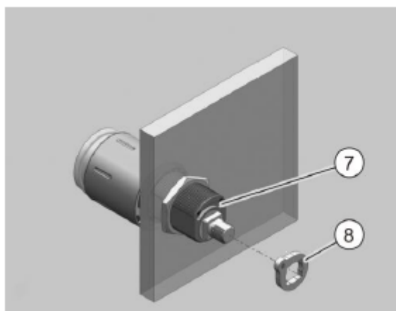
Fig. 148: Attaching the lever travel limiter
