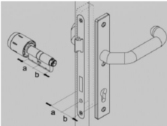
Fig. 106: Measuring the thickness
