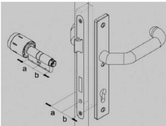
Fig. 116: Measuring the thickness
