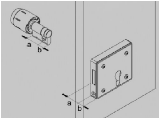
Fig. 129: Measuring the thickness
