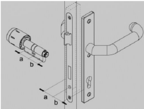
Fig. 26: Measuring the thickness
