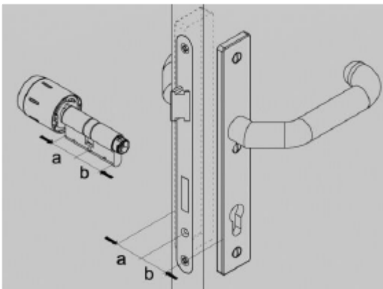
Fig. 120: Measuring the thickness
