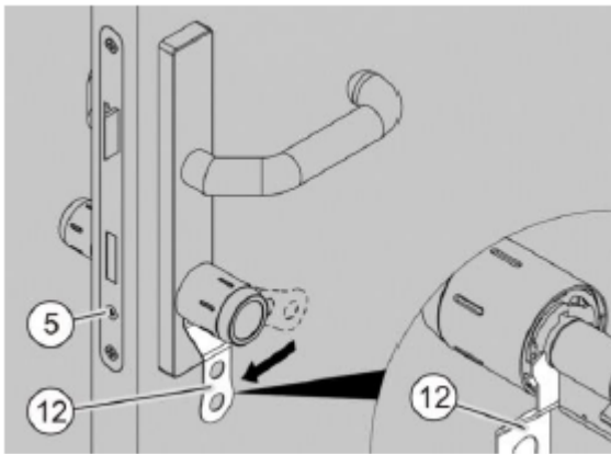
Fig. 66: Locking the bayonet lock
