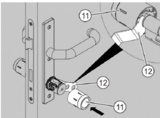
Fig. 79: Sliding on the knob sleeve
