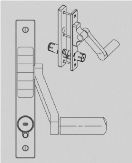
Fig. 82: Example of a panic bar
