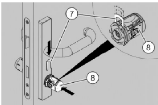
Fig. 95: Assembling the electronic knob
