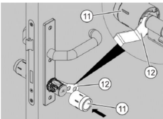
Fig. 64: Sliding on the knob sleeve
