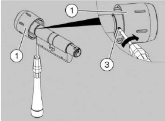
Fig. 92: Tightening the inner knob
