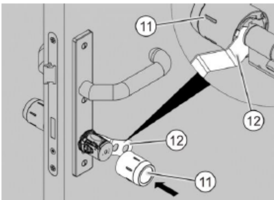
Fig. 97: Sliding on the knob sleeve
