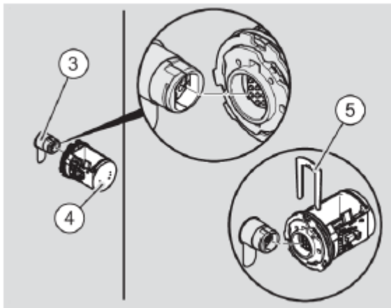
Fig. 134: Assembling the electronic knob
