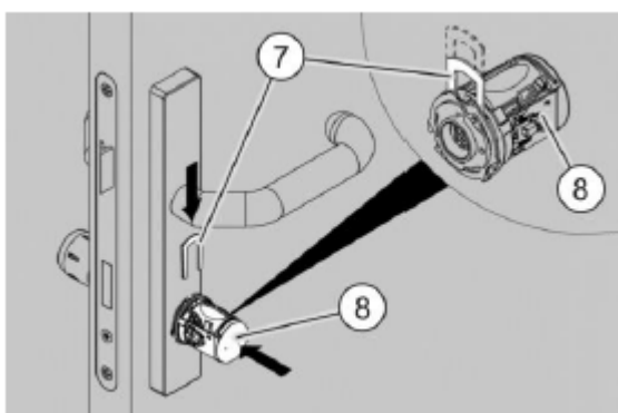
Fig. 21: Assembling the electronic knob
