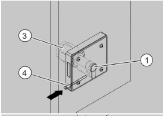
Fig. 131: Securing the cylinder
