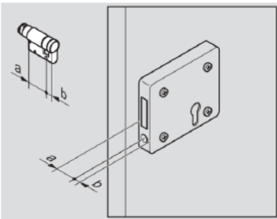
Fig. 132: Measuring the thickness
