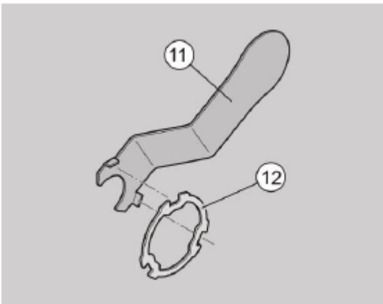
Fig. 50: Attaching the knob tool
