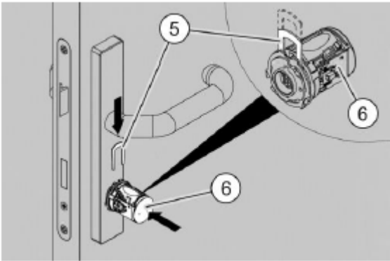
Fig. 109: Assembling the electronic knob
