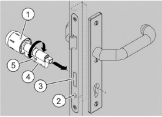
Fig. 27: Inserting the cylinder
