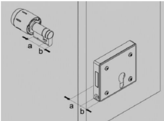
Fig. 140: Measuring the thickness
