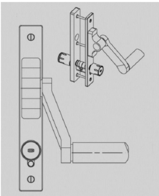
Fig. 105: Installation situation for the panic bar
