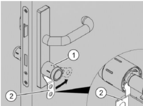
Fig. 160: Unlocking the bayonet lock
