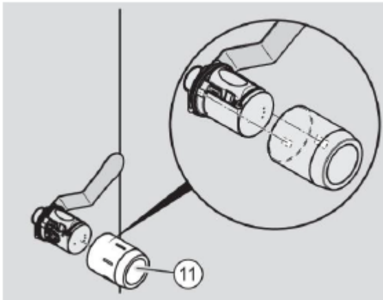
Fig. 137: Pushing on the knob sleeve
