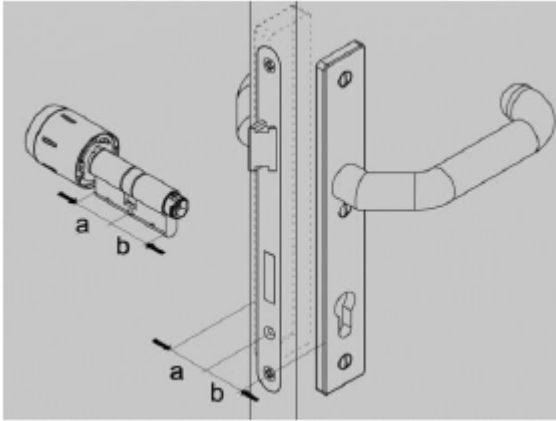
Fig. 90: Measuring the thickness
