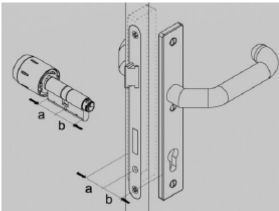
Fig. 67: Measuring the thickness
