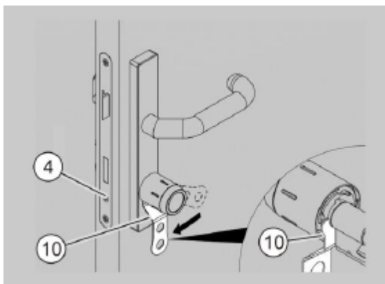
Fig. 127: Locking the bayonet lock
