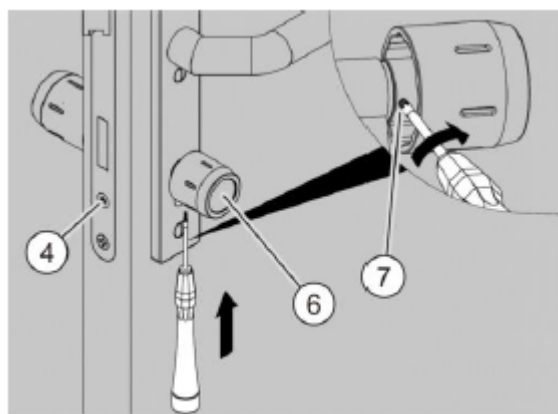
Fig. 71: Securing the inner knob
