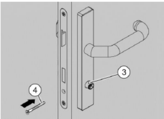
Fig. 122: Securing the cylinder
