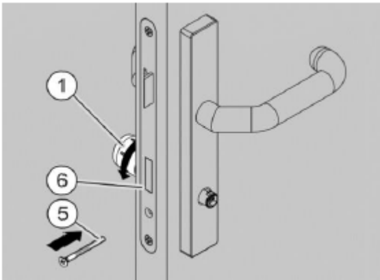
Fig. 61: Aligning the locking nose
