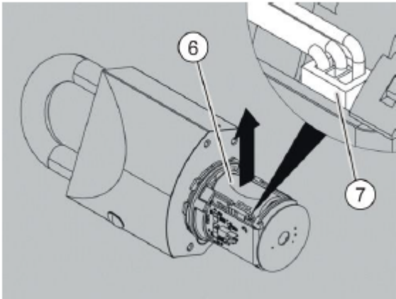
Fig. 172: Inserting the battery pack
