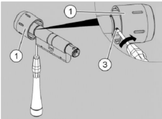
Fig. 74: Tightening the inner knob
