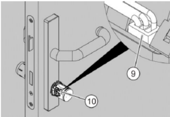
Fig. 96: Connecting the battery
