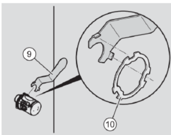
Fig. 136: Sliding on the knob sleeve
