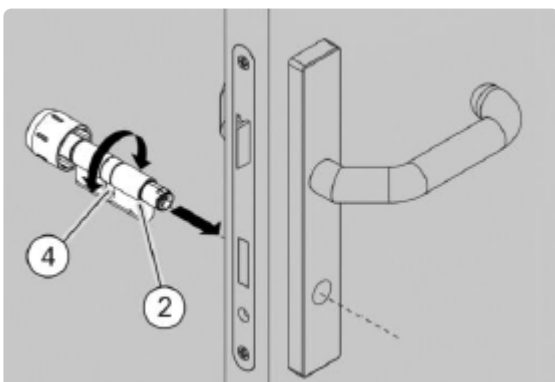
Fig. 19: Inserting the cylinder
