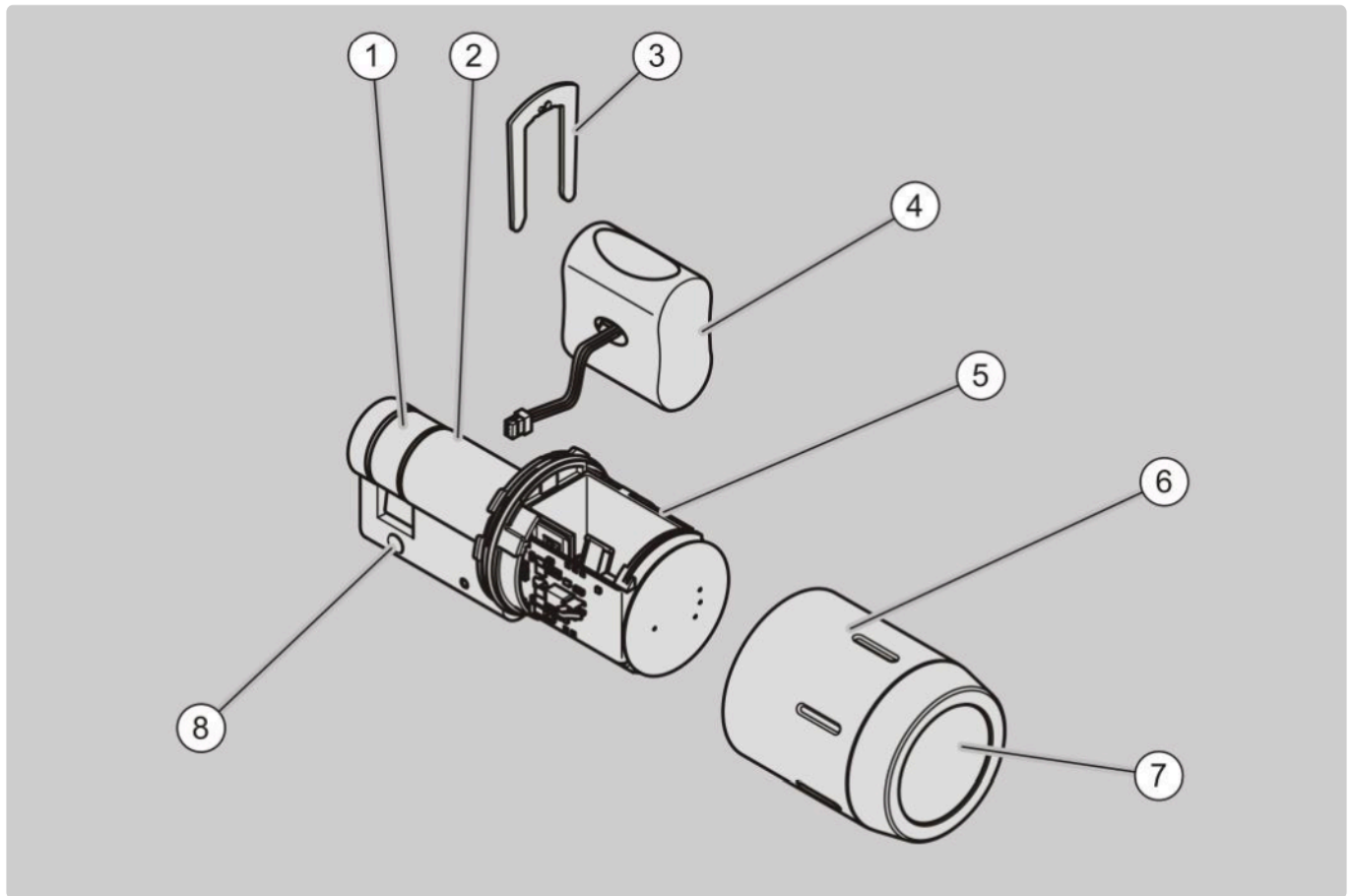
Fig. 3: Overview of the half-cylinder's components
