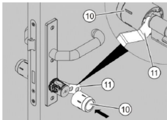
Fig. 41: Sliding on the knob sleeve
