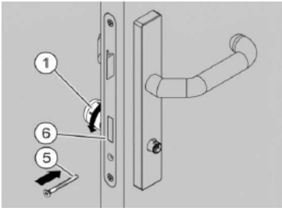
Fig. 94: Aligning the locking nose
