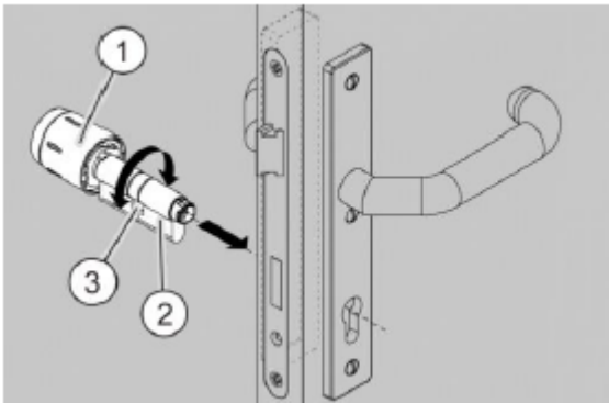
Fig. 45: Aligning the locking nose
