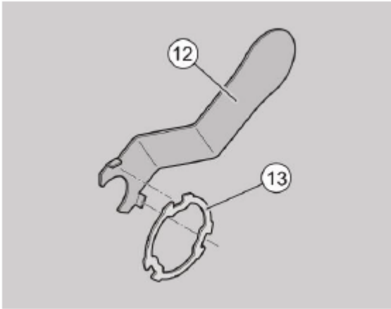
Fig. 24: Attaching the knob tool
