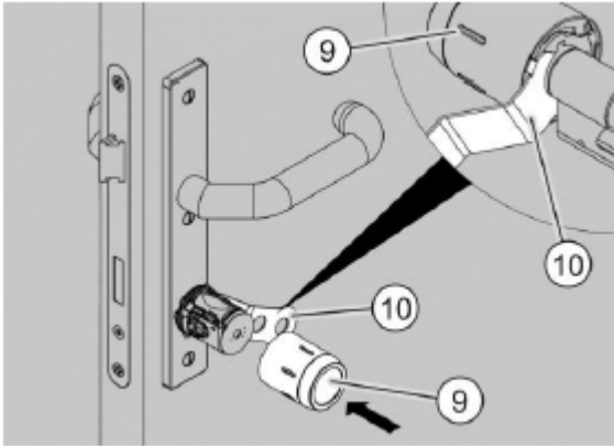
Fig. 111: Sliding on the knob sleeve
