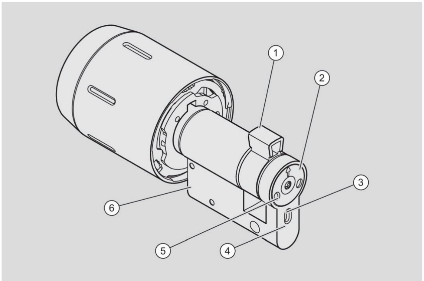
Fig. 4: Overview of the Pro MiWE half-cylinder's components
