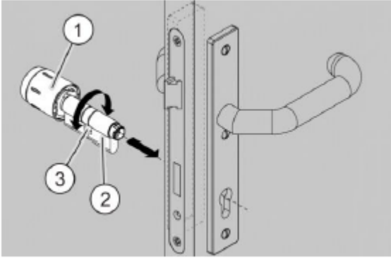
Fig. 12: Inserting the cylinder
