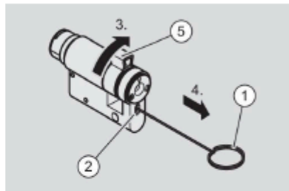
Fig. 10: Engaging the driver
