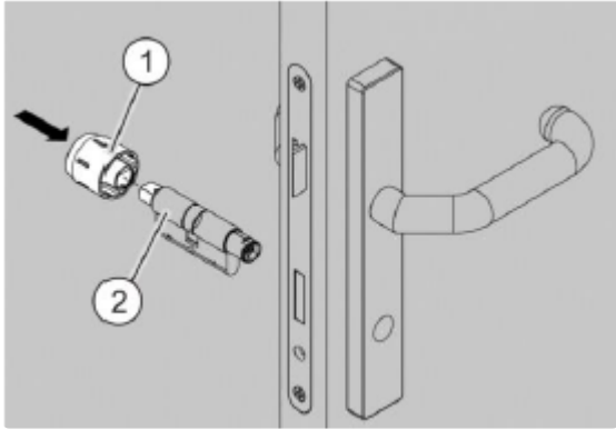
Fig. 17: Fitting the inner knob
