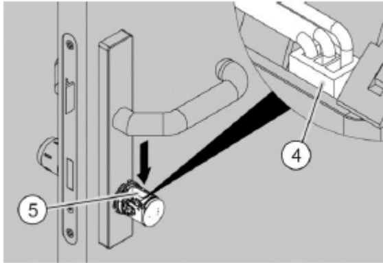
Fig. 162: Removing the battery pack
