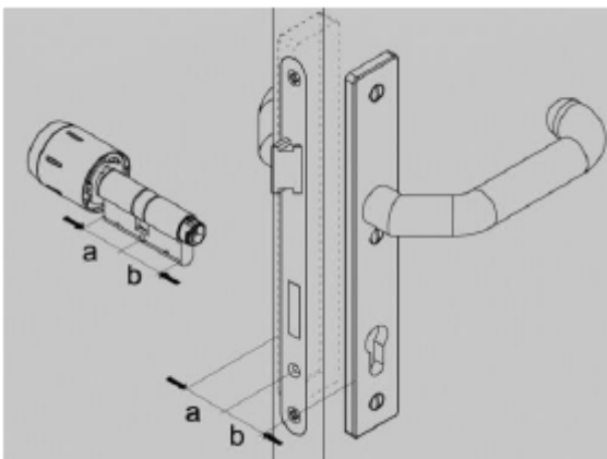
Fig. 16: Measuring the thickness
