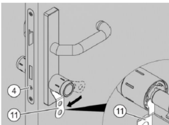
Fig. 51: Locking the bayonet lock
