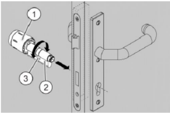
Fig. 53: Inserting the cylinder
