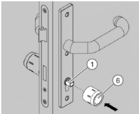
Fig. 86: Fitting the inner knob
