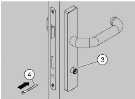
Fig. 108: Securing the cylinder
