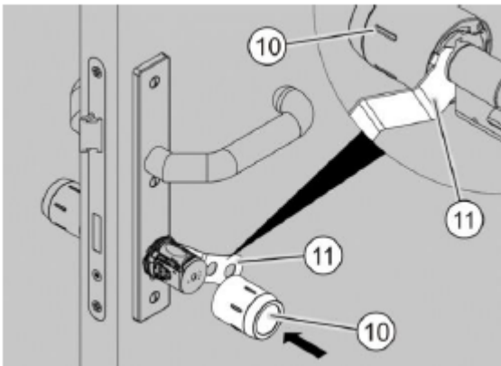
Fig. 49: Sliding on the knob sleeve
