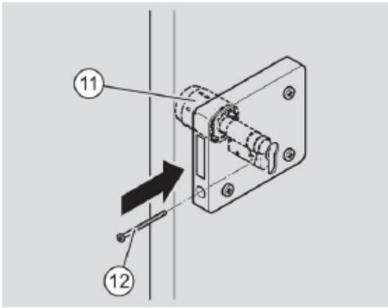
Fig. 139: Securing the cylinder
