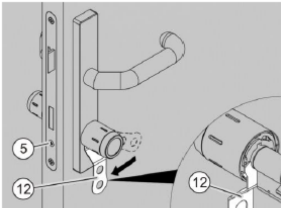
Fig. 25: Locking the bayonet lock
