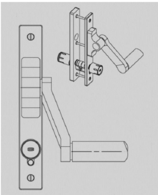
Fig. 119: Installation situation for the panic bar
