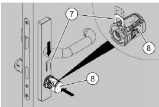
Fig. 77: Assembling the electronic knob
