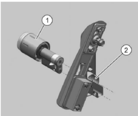
Fig. 143: Inserting the cylinder
