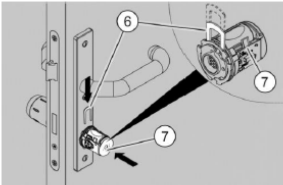
Fig. 47: Assembling the electronic knob
