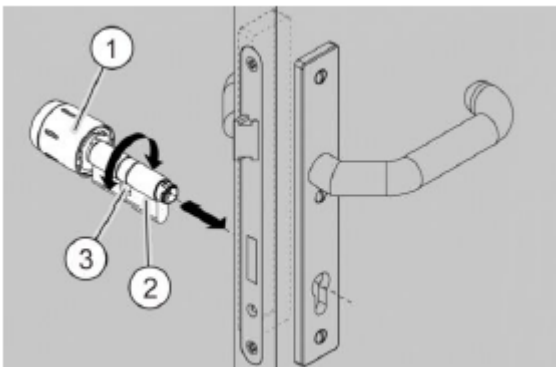
Fig. 84: Inserting the cylinder
