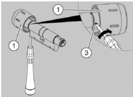
Fig. 18: Tightening the inner knob
