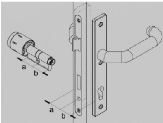
Fig. 52: Measuring the thickness
