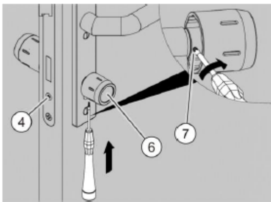
Fig. 56: Securing the inner knob
