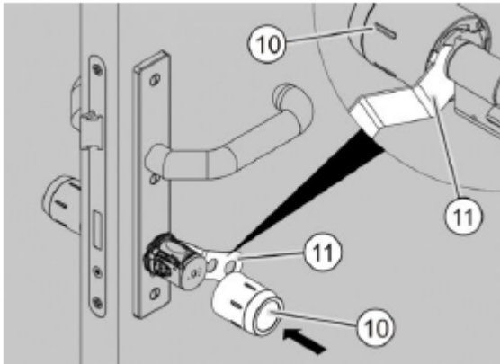
Fig. 125: Sliding on the knob sleeve
