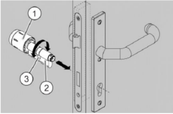
Fig. 68: Inserting the cylinder
