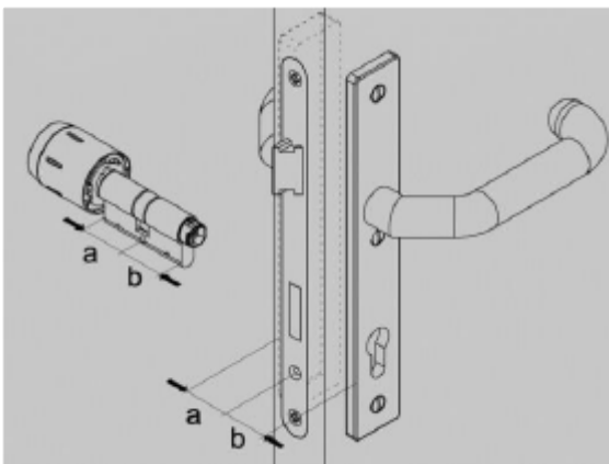
Fig. 57: Measuring the thickness
