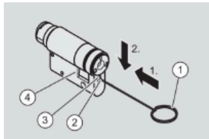
Fig. 9: Unlocking the driver
