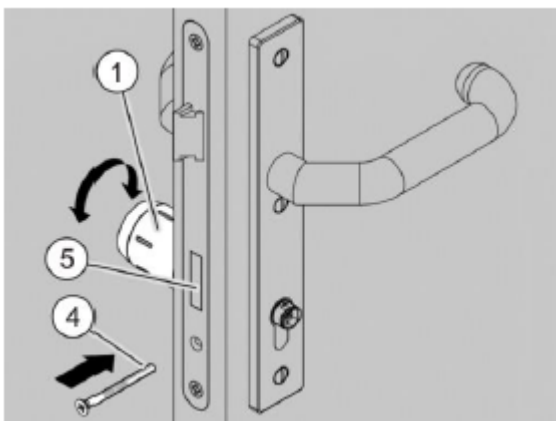
Fig. 46: Inserting the cylinder
