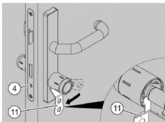
Fig. 43: Locking the bayonet lock
