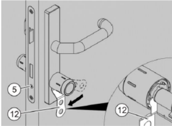
Fig. 81: Locking the bayonet lock
