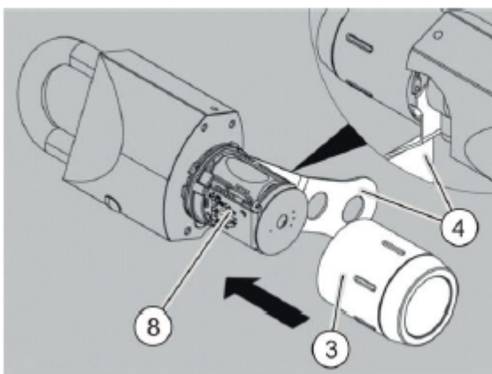
Fig. 173: Assembling the knob sleeve
