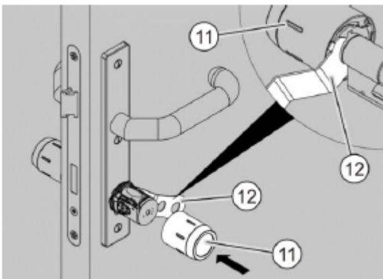
Fig. 23: Sliding on the knob sleeve
