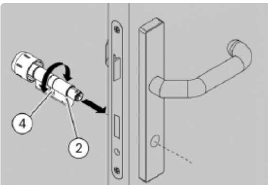
Fig. 75: Inserting the cylinder
