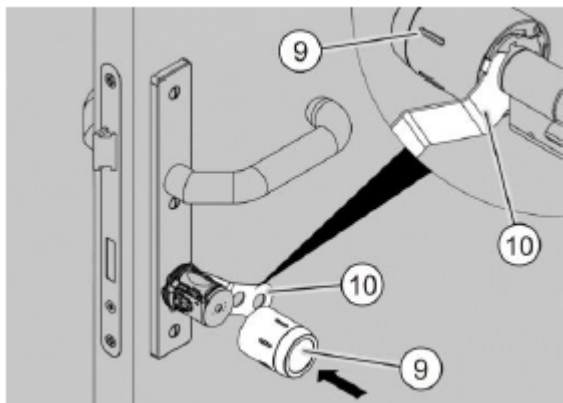
Fig. 33: Attaching the knob sleeve
