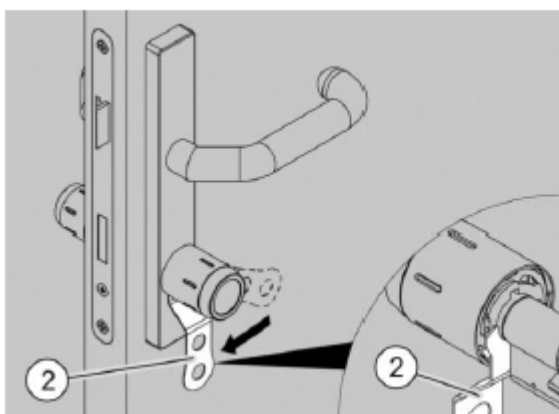
Fig. 166: Locking the bayonet lock
