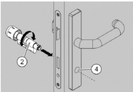
Fig. 93: Inserting the cylinder
