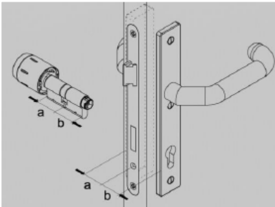
Fig. 102: Measuring the thickness
