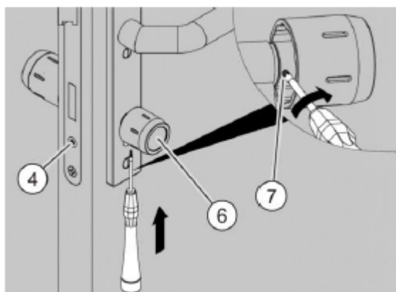
Fig. 87: Securing the inner knob
