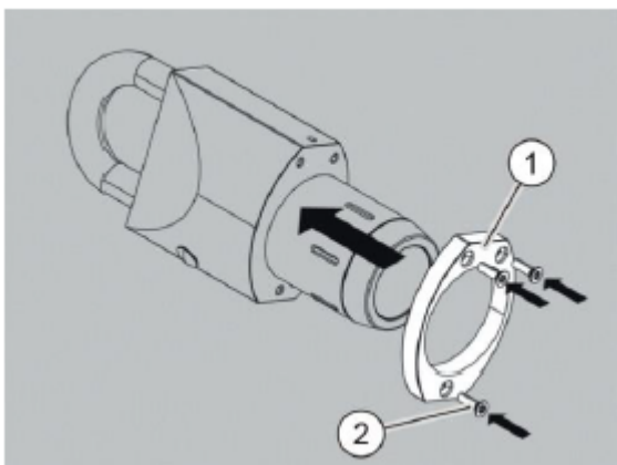
Fig. 176: Assembling the protective cap
